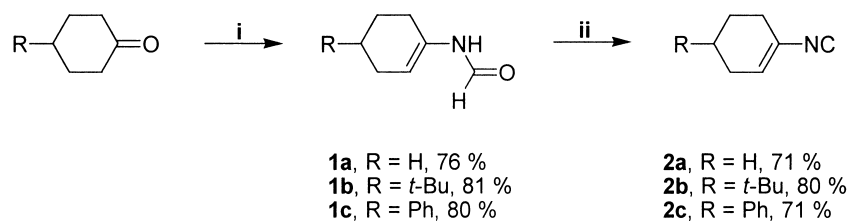
Scheme 2. Synthesis of vinylic isocyanides 2a–c . Reagents and conditions: (i) formamide, H 2 SO 4 , toluene, Dean–Stark conditions; (ii) phosgene, NEt 3 , 0 °C.
