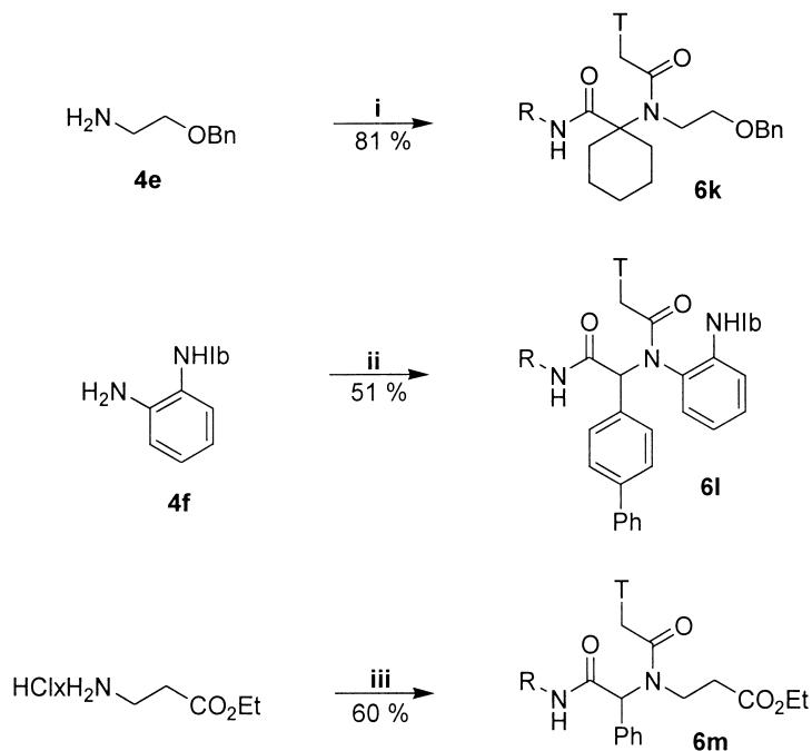
Scheme 3. Examples of totally protected PNA-monomers (R = 4- tert -butyl-cyclohex-1-enyl). Reagents and conditions: (i) cyclohexanone, 5a , 2b , MeOH, rt; (ii) 4-biphenylcarbaldehyde, 5a , 2b , MeOH, rt; (iii) benzaldehyde, 5a , 2b , triethylamine, MeOH, rt.
