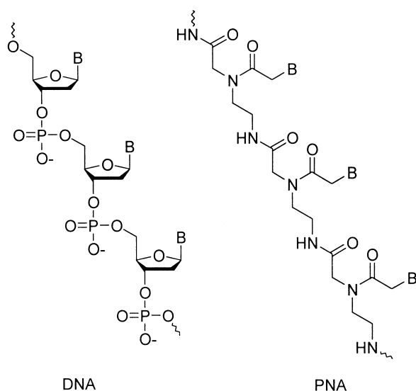
Figure 1. B = adenine, cytosine, guanine, thymine.
