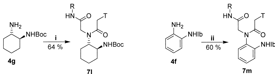
Scheme 4. Employment of cyclic diamines in the 4CC; only one enantiomer for racemic 7l is shown ( R = 4 -methoxy-2-nitro-phenyl). Reagents and conditions: (i) formaldehyde, 5a , 3a , MeOH, rt; (ii) formaldehyde, 5a , 3a , MeOH, rt.
