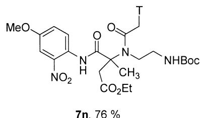
Figure 2. Polyfunctional PNA-monomer ( R = 4 -methoxy-2-nitro-phenyl).
