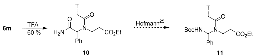
Scheme 6. Synthesis of a 'retro-inverso' PNA-monomer.
