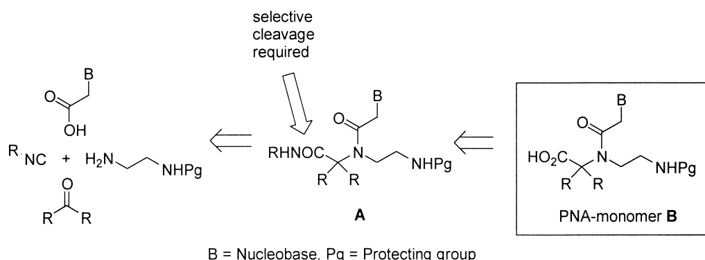
Scheme 1. Ugi 4CC and regioselective hydrolysis to mono-protected PNA-monomers.
