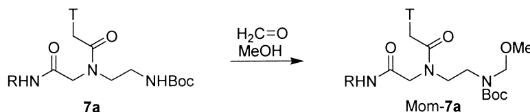
Scheme 5. Methoxymethylenation of aeg-monomers ( R = 4 -methoxy-2-nitro-phenyl).
